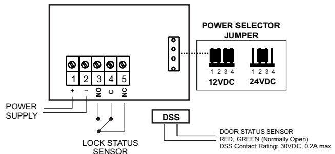
Figure 2. FEM6600M/FEM6600DM
