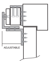
'L' & 'Z' BRACKET ARRANGEMENT
