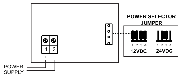
Figure 1. FEM6600/FEM6600D
